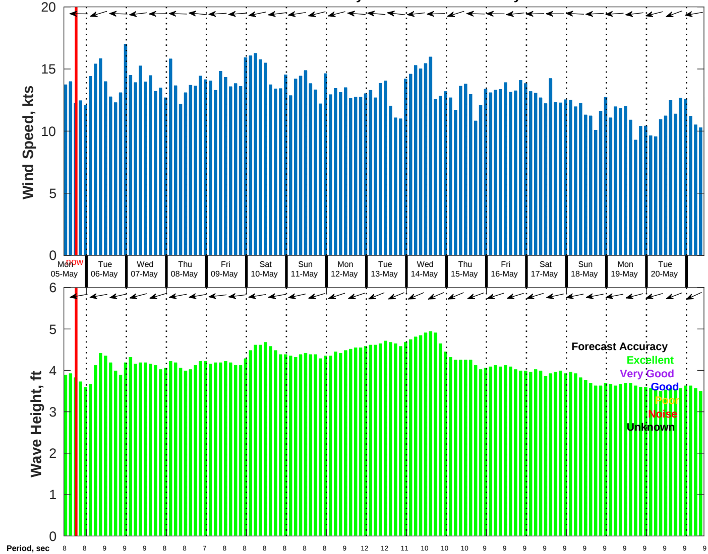
Wind & Wave Forecast for NDBC 52211 from 04-May-2025 10:00:00 to 20-May-2025 10:00:00
