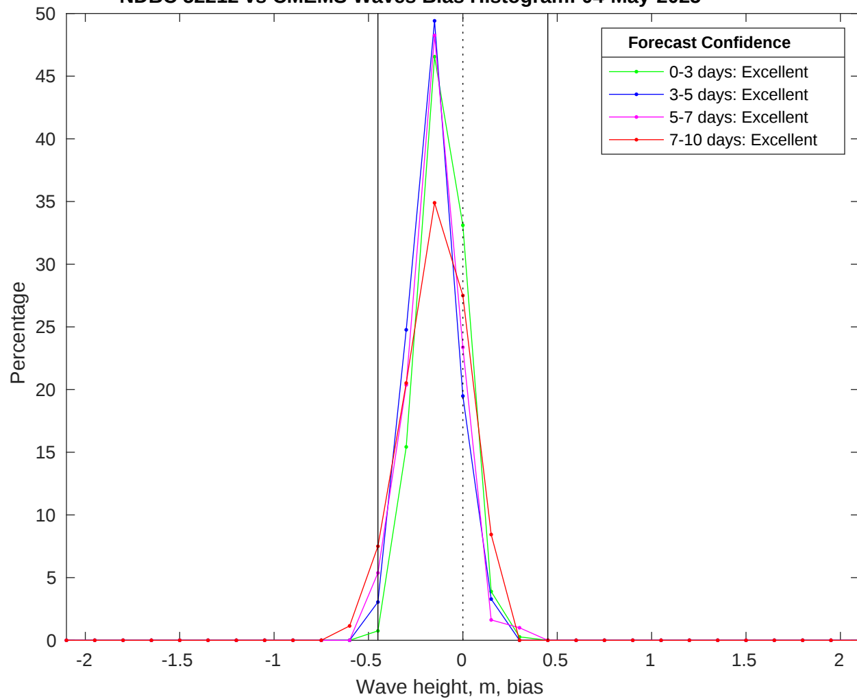
NDBC 52212 vs CMEMS Waves Bias Histogram: 04-May-2025
