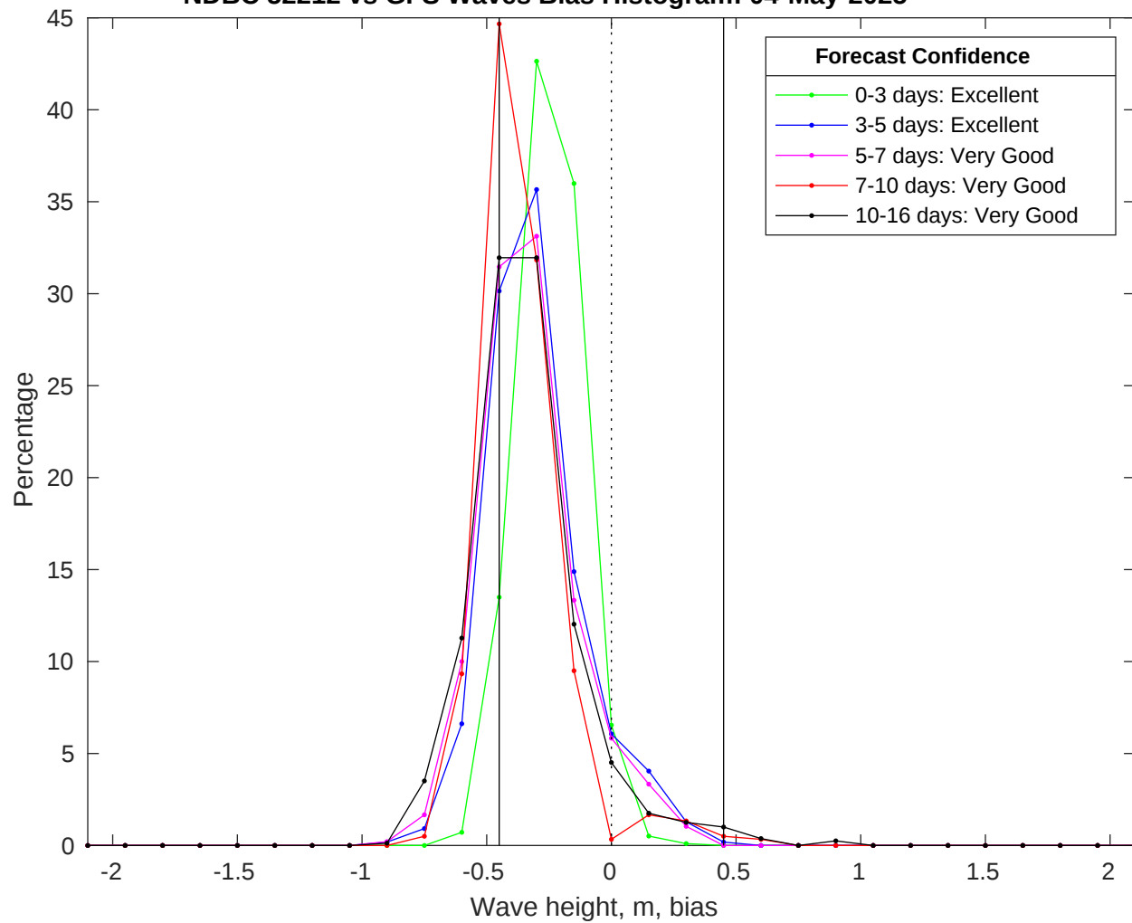
NDBC 52212 vs GFS Waves Bias Histogram: 04-May-2025
