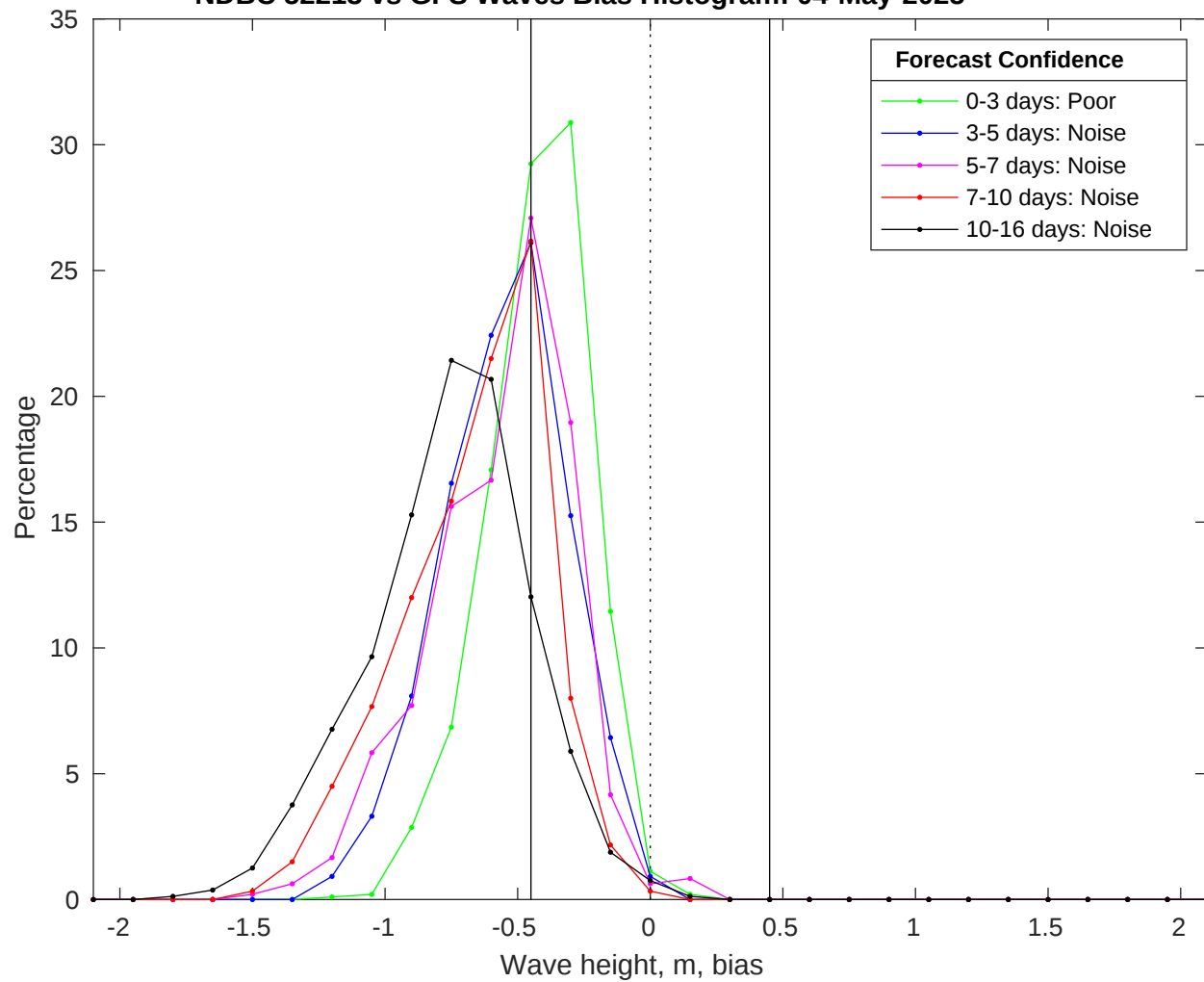
NDBC 52213 vs GFS Waves Bias Histogram: 04-May-2025
