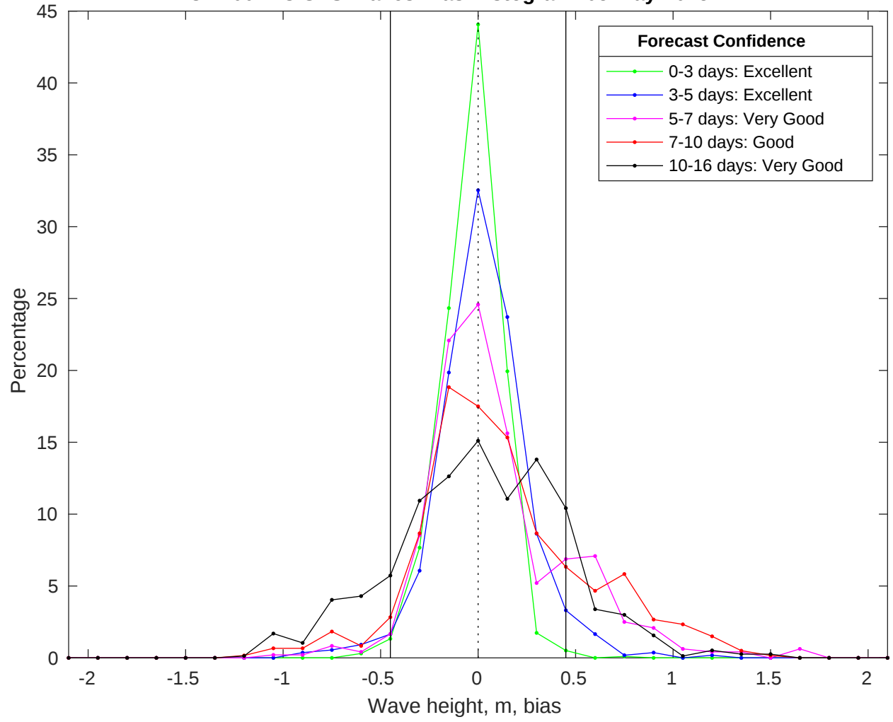
NDBC 41004 vs GFS Waves Bias Histogram: 05-May-2025
