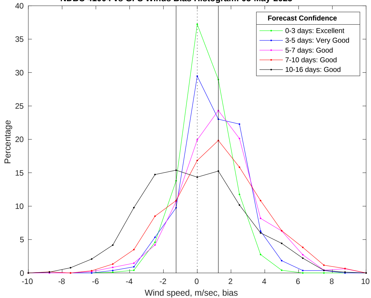
NDBC 41004 vs GFS Winds Bias Histogram: 05-May-2025
