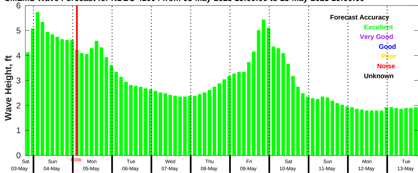
CMEMS Wave Forecast for NDBC 41004 from 03-May-2025 19:00:00 to 13-May-2025 19:00:00
