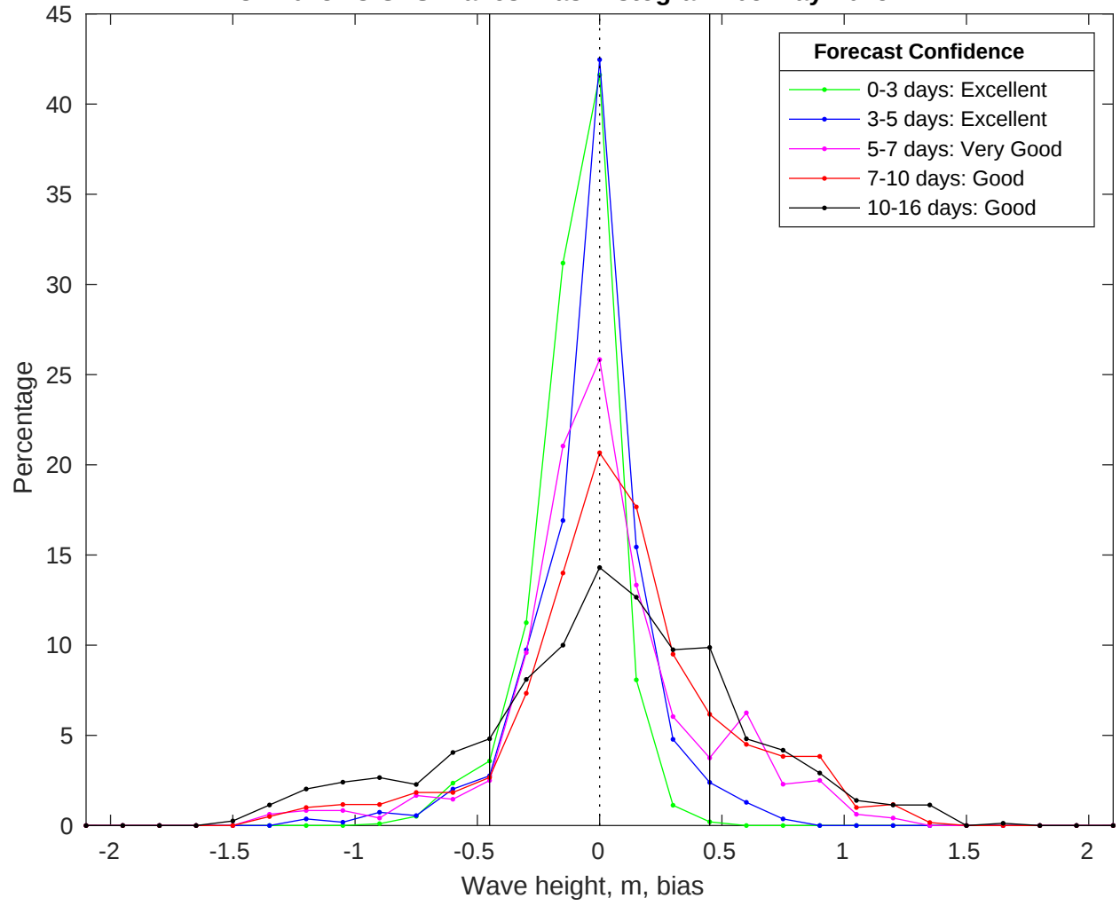
NDBC 41013 vs GFS Waves Bias Histogram: 05-May-2025
