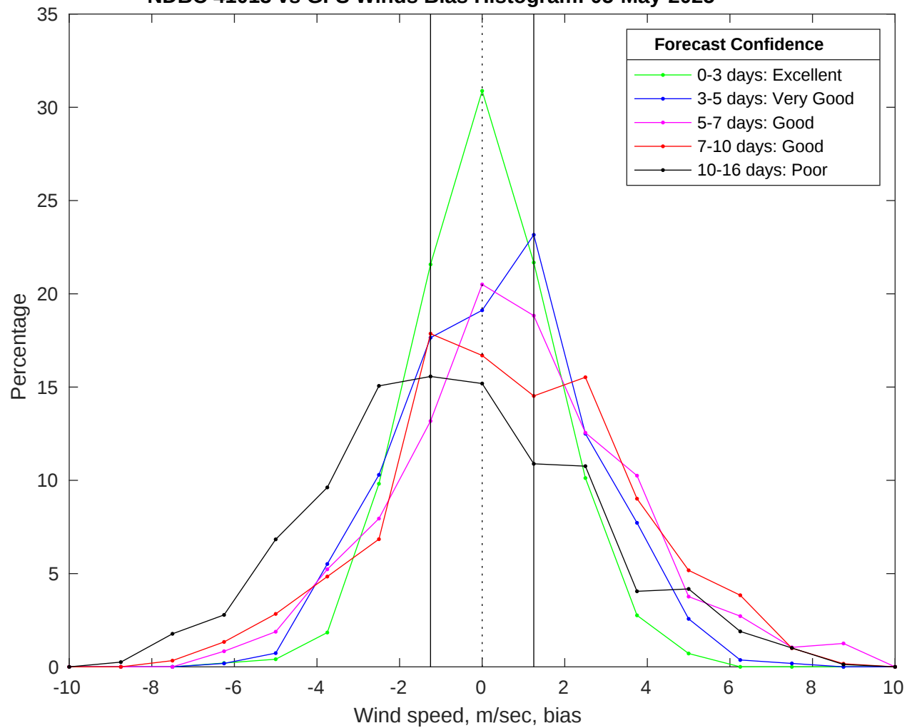
NDBC 41013 vs GFS Winds Bias Histogram: 05-May-2025
