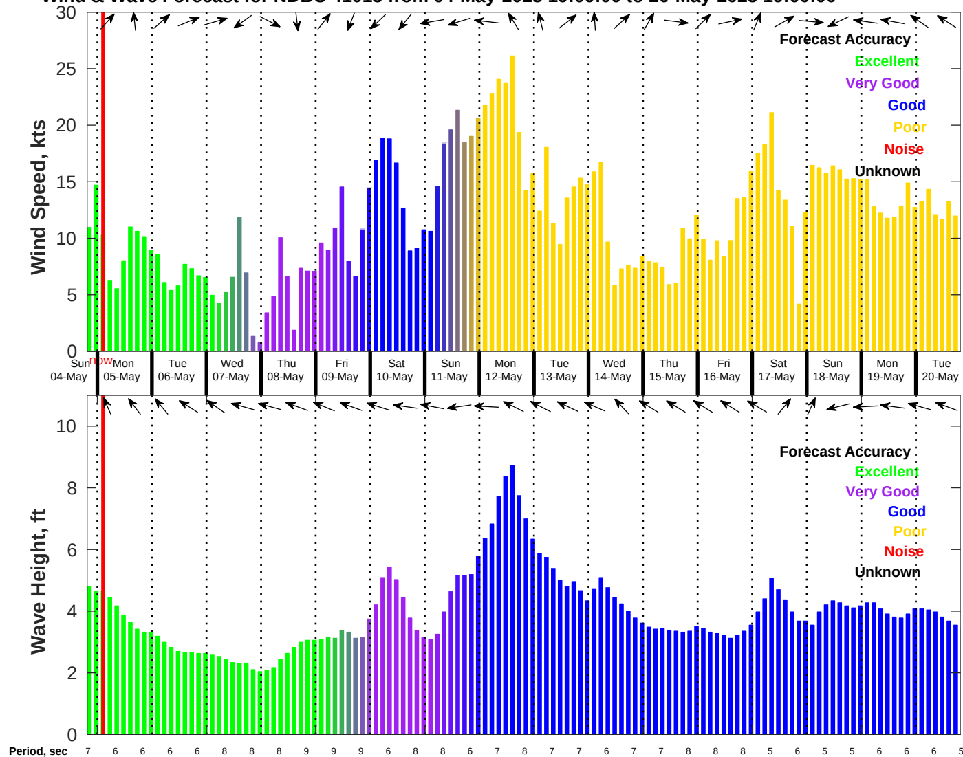
Wind & Wave Forecast for NDBC 41013 from 04-May-2025 19:00:00 to 20-May-2025 19:00:00
