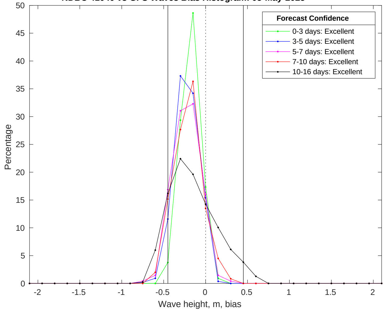
NDBC 41040 vs GFS Waves Bias Histogram: 05-May-2025
