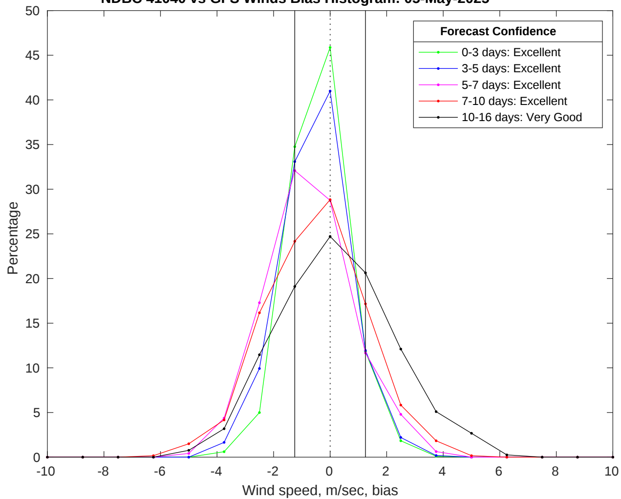
NDBC 41040 vs GFS Winds Bias Histogram: 05-May-2025
