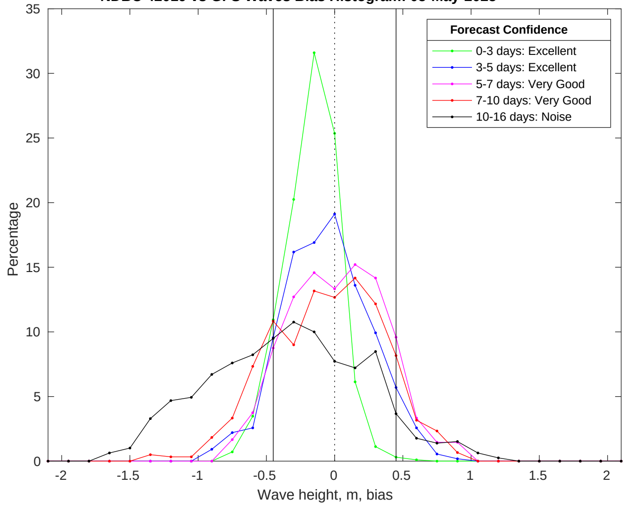
NDBC 42019 vs GFS Waves Bias Histogram: 05-May-2025
