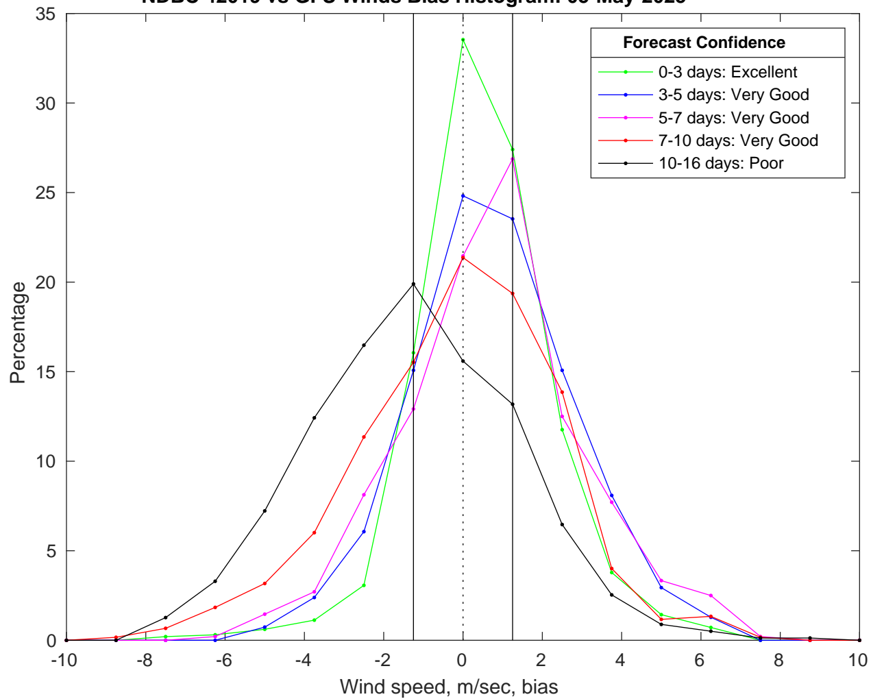
NDBC 42019 vs GFS Winds Bias Histogram: 05-May-2025
