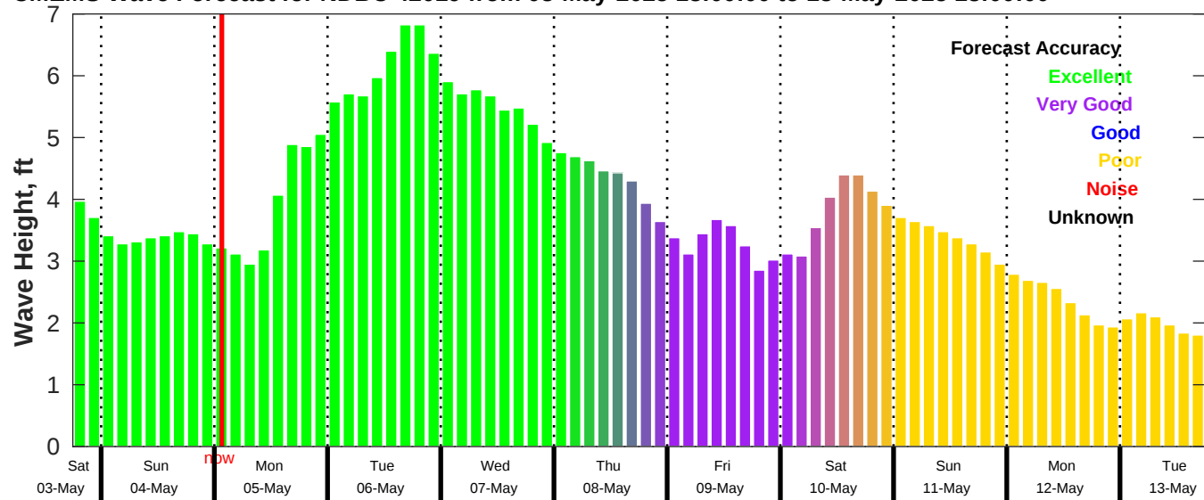
CMEMS Wave Forecast for NDBC 42019 from 03-May-2025 18:00:00 to 13-May-2025 18:00:00
