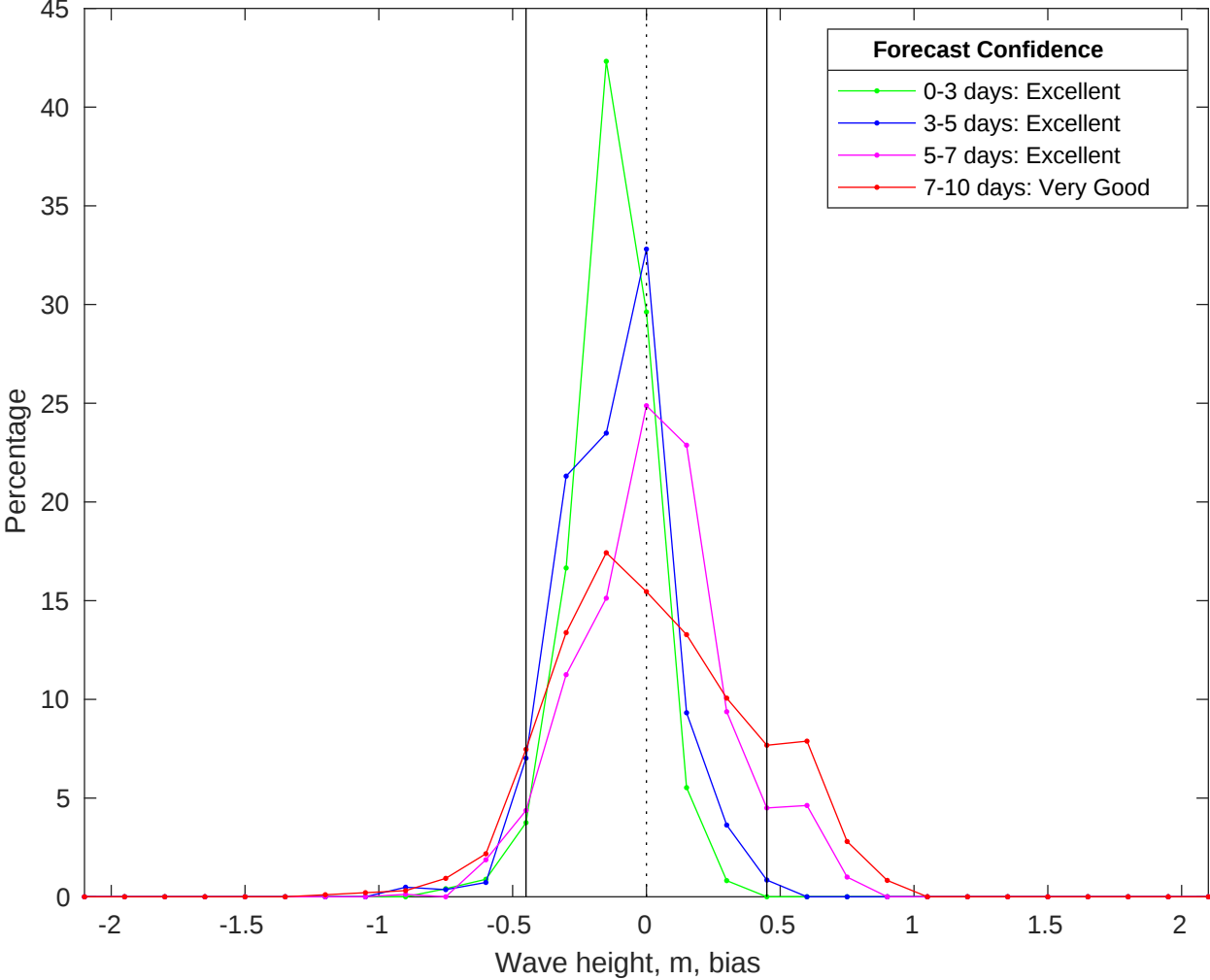
NDBC 42020 vs CMEMS Waves Bias Histogram: 05-May-2025
