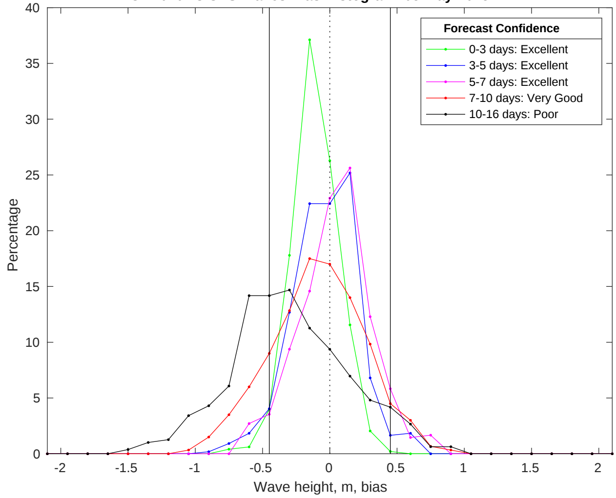
NDBC 42020 vs GFS Waves Bias Histogram: 05-May-2025
