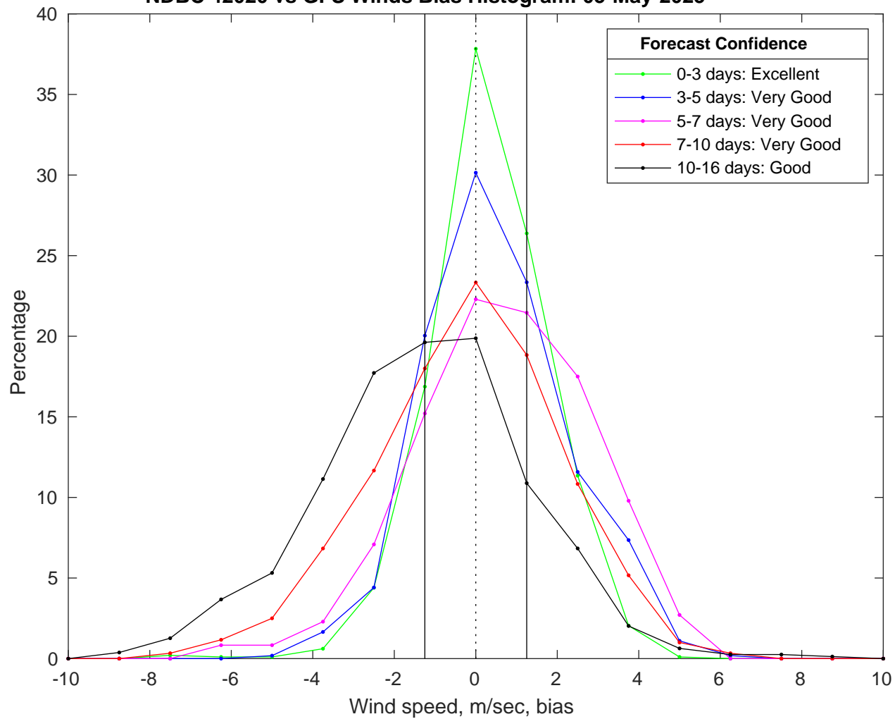
NDBC 42020 vs GFS Winds Bias Histogram: 05-May-2025
