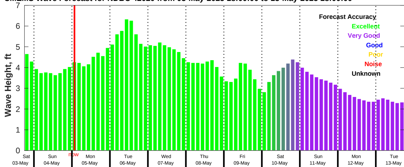
CMEMS Wave Forecast for NDBC 42020 from 03-May-2025 18:00:00 to 13-May-2025 18:00:00
