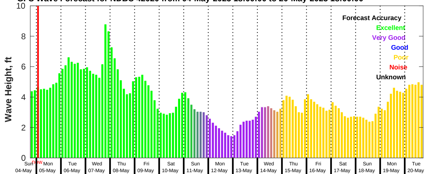
GFS Wave Forecast for NDBC 42020 from 04-May-2025 18:00:00 to 20-May-2025 18:00:00
