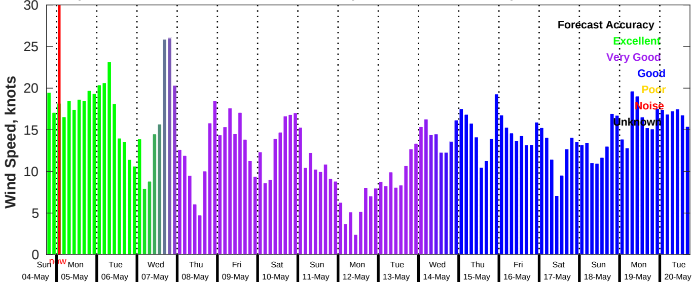
GFS Wind Speed Forecast for NDBC 42020 from 04-May-2025 18:00:00 to 20-May-2025 18:00:00
