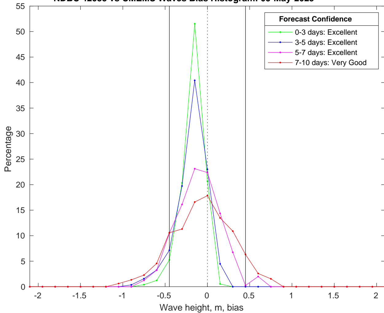
NDBC 42035 vs CMEMS Waves Bias Histogram: 05-May-2025
