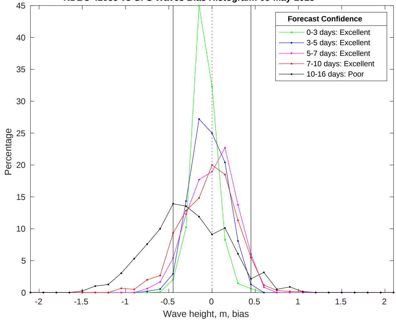
NDBC 42035 vs GFS Waves Bias Histogram: 05-May-2025
