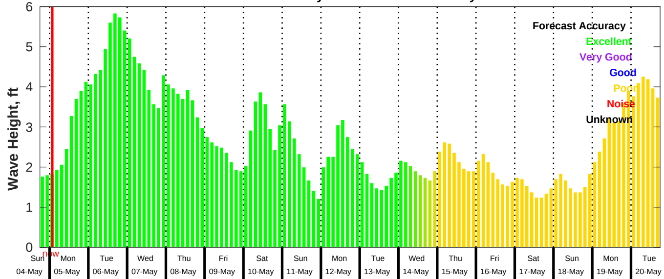
GFS Wave Forecast for NDBC 42035 from 04-May-2025 18:00:00 to 20-May-2025 18:00:00
