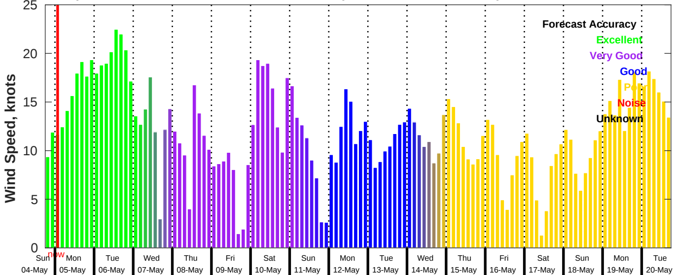
GFS Wind Speed Forecast for NDBC 42035 from 04-May-2025 18:00:00 to 20-May-2025 18:00:00
