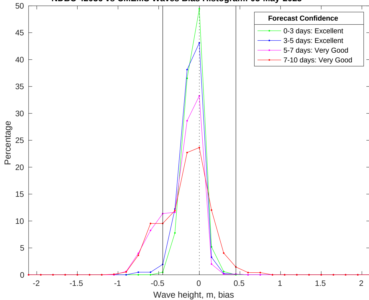
NDBC 42036 vs CMEMS Waves Bias Histogram: 05-May-2025
