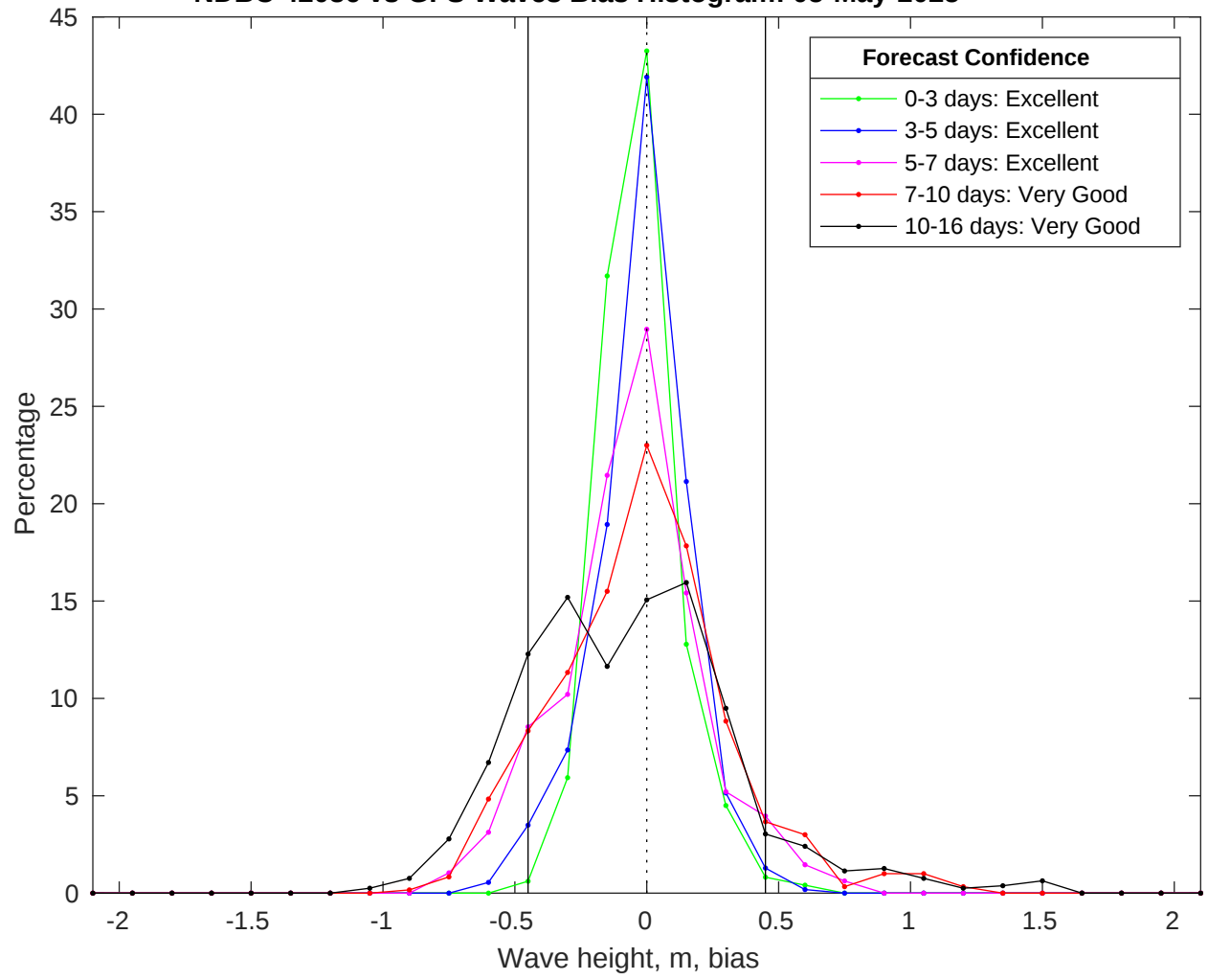
NDBC 42036 vs GFS Waves Bias Histogram: 05-May-2025
