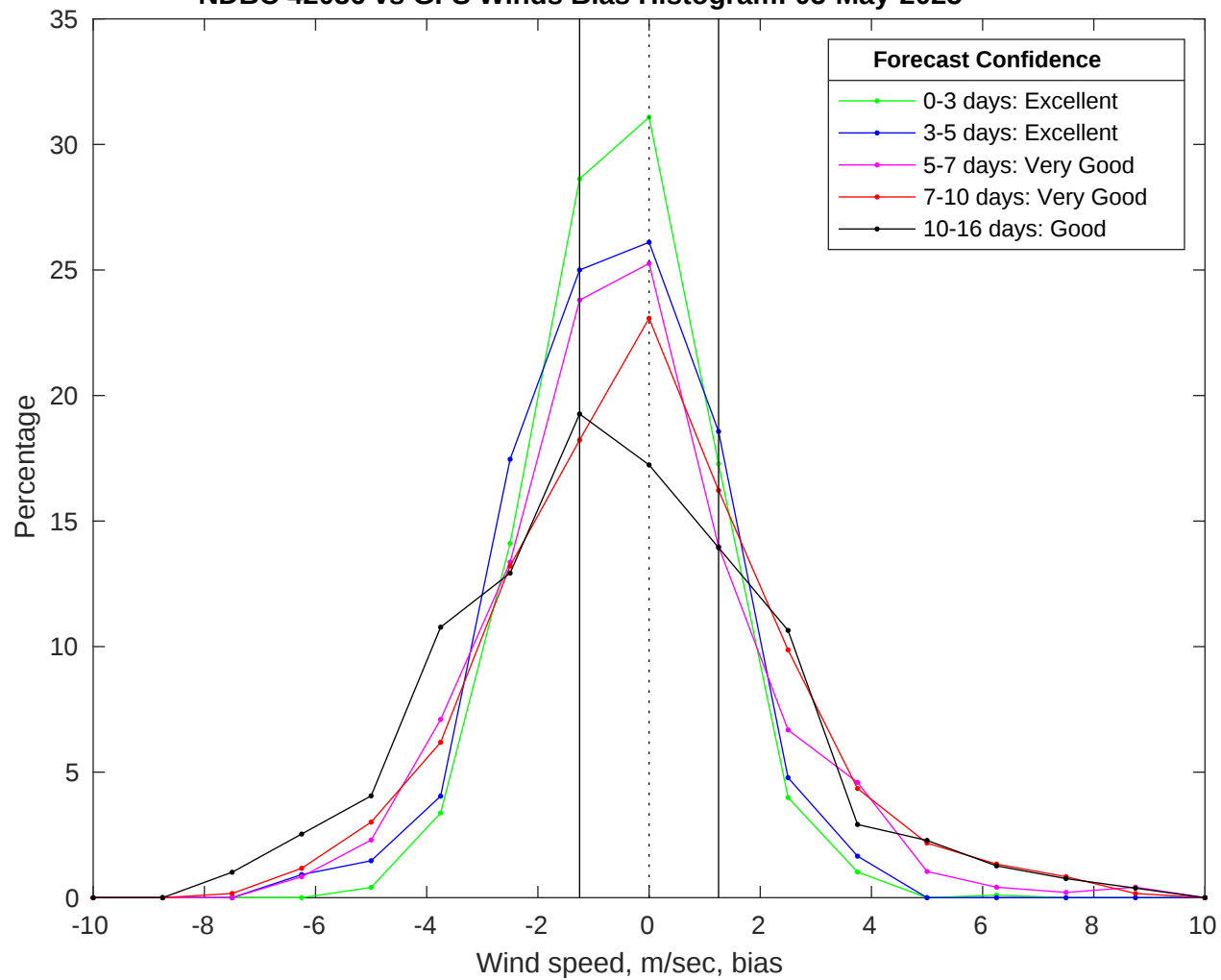
NDBC 42036 vs GFS Winds Bias Histogram: 05-May-2025
