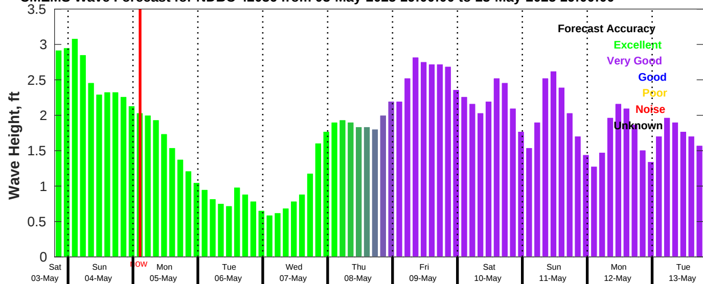
CMEMS Wave Forecast for NDBC 42036 from 03-May-2025 19:00:00 to 13-May-2025 19:00:00
