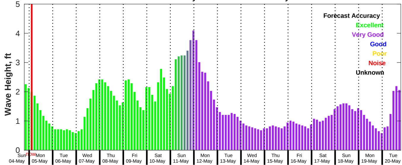
GFS Wave Forecast for NDBC 42036 from 04-May-2025 19:00:00 to 20-May-2025 19:00:00
