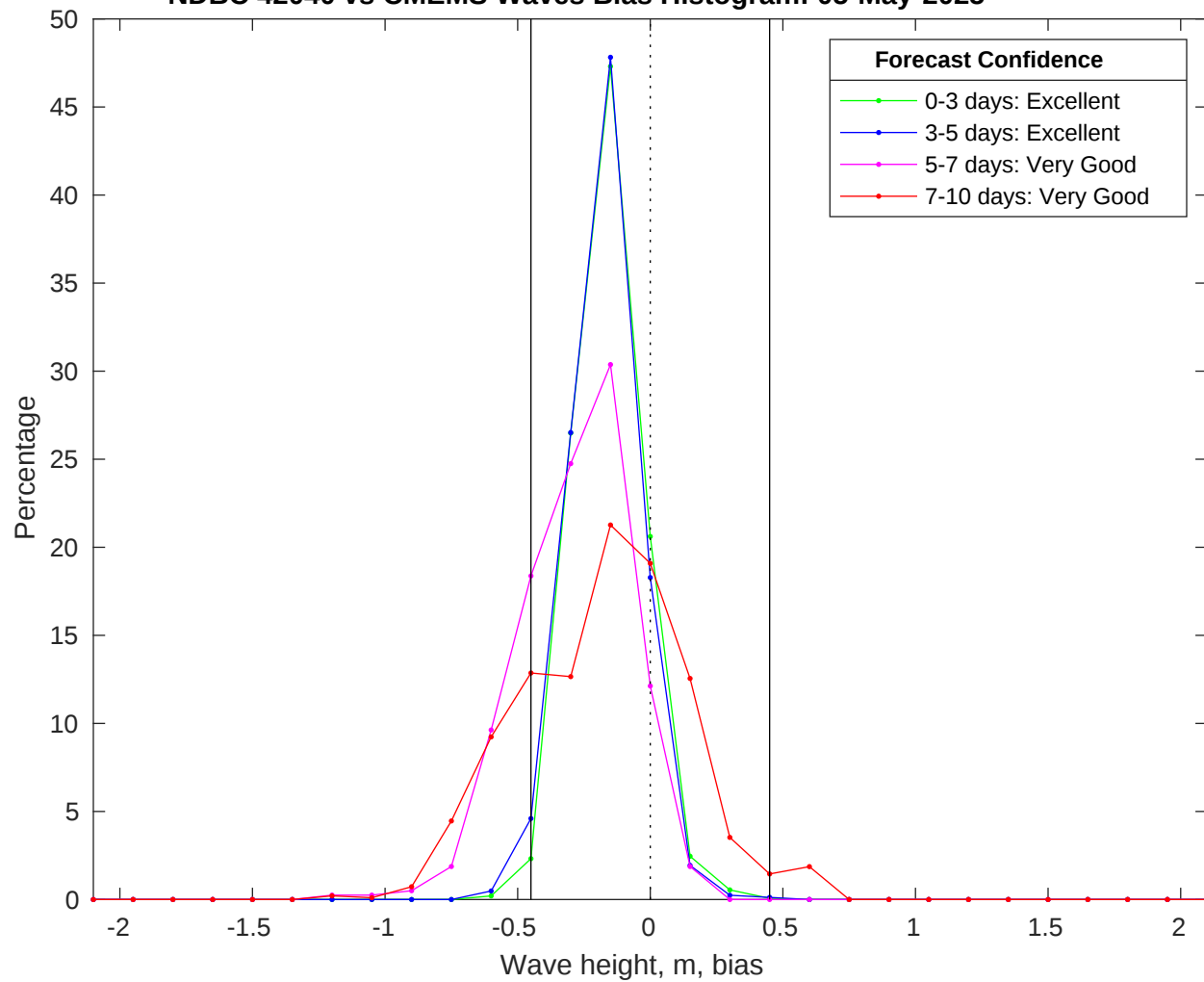
NDBC 42040 vs CMEMS Waves Bias Histogram: 05-May-2025
