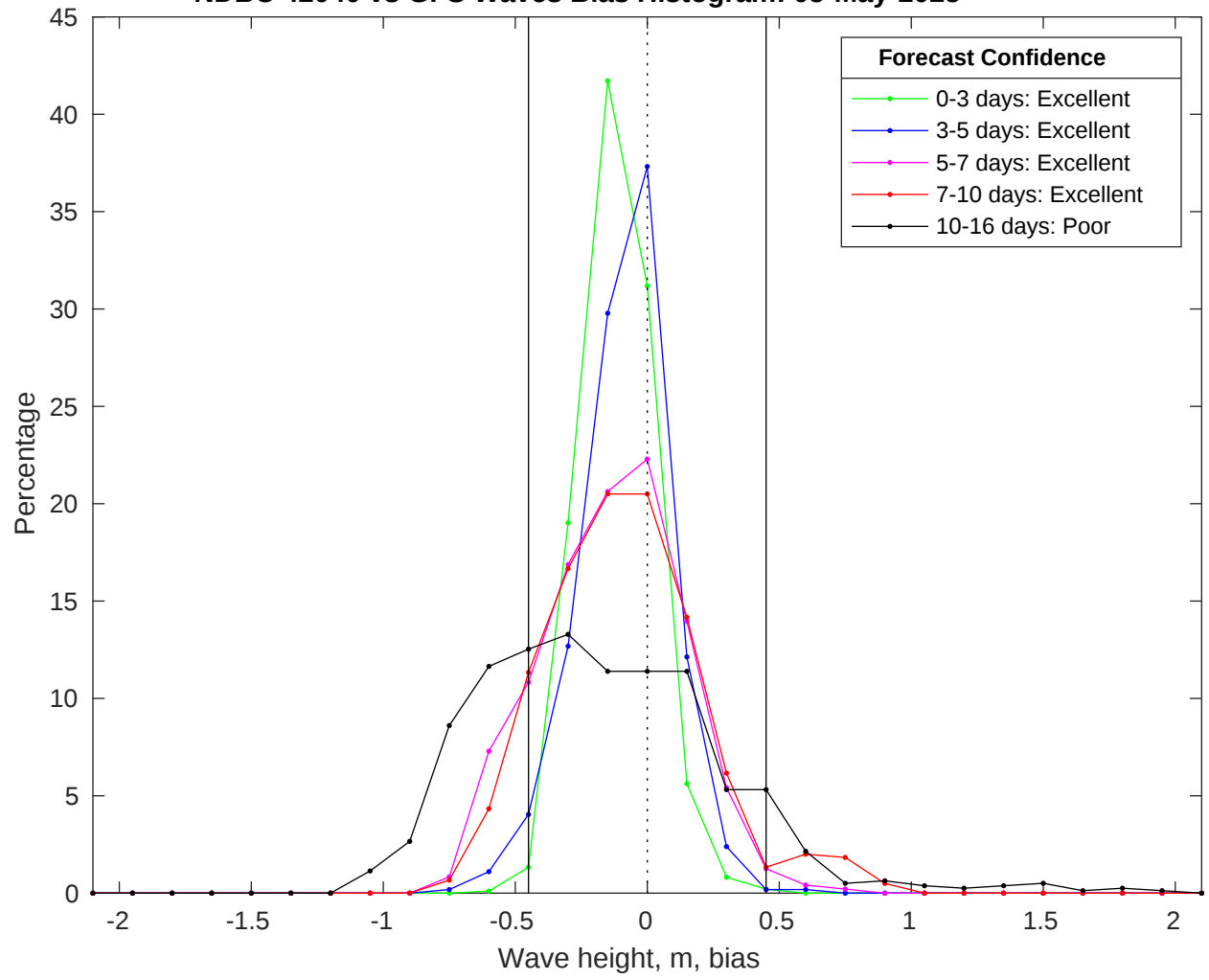
NDBC 42040 vs GFS Waves Bias Histogram: 05-May-2025
