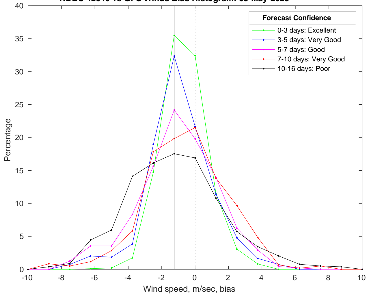
NDBC 42040 vs GFS Winds Bias Histogram: 05-May-2025
