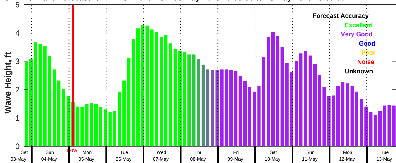
CMEMS Wave Forecast for NDBC 42040 from 03-May-2025 19:00:00 to 13-May-2025 19:00:00
