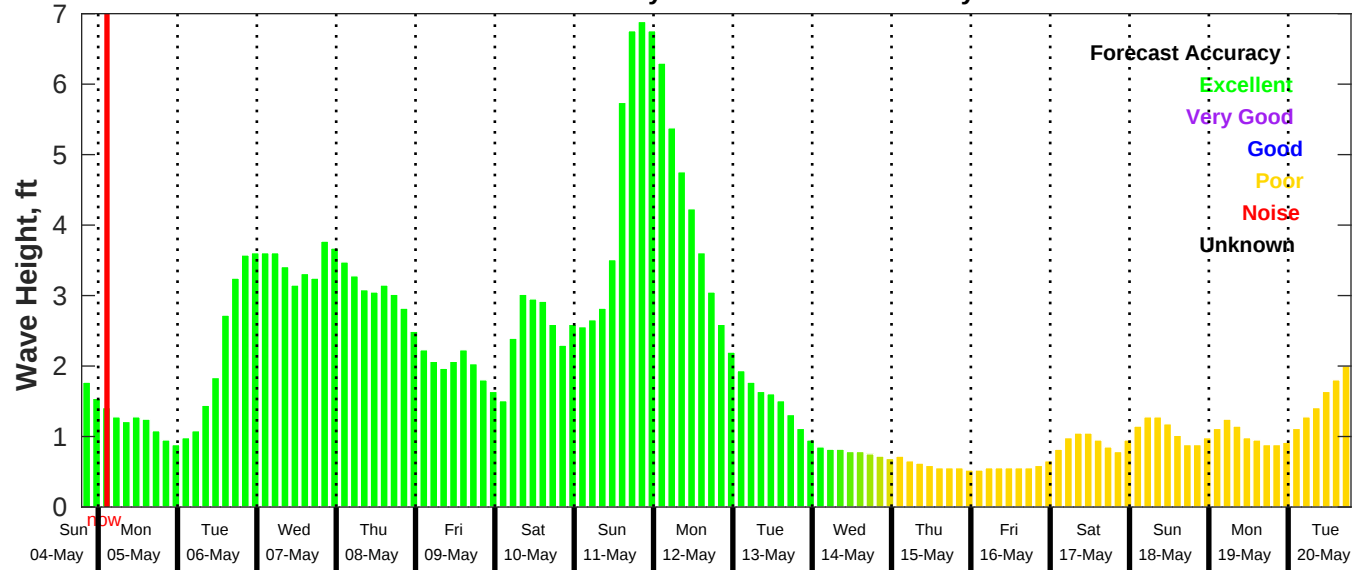
GFS Wave Forecast for NDBC 42040 from 04-May-2025 19:00:00 to 20-May-2025 19:00:00
