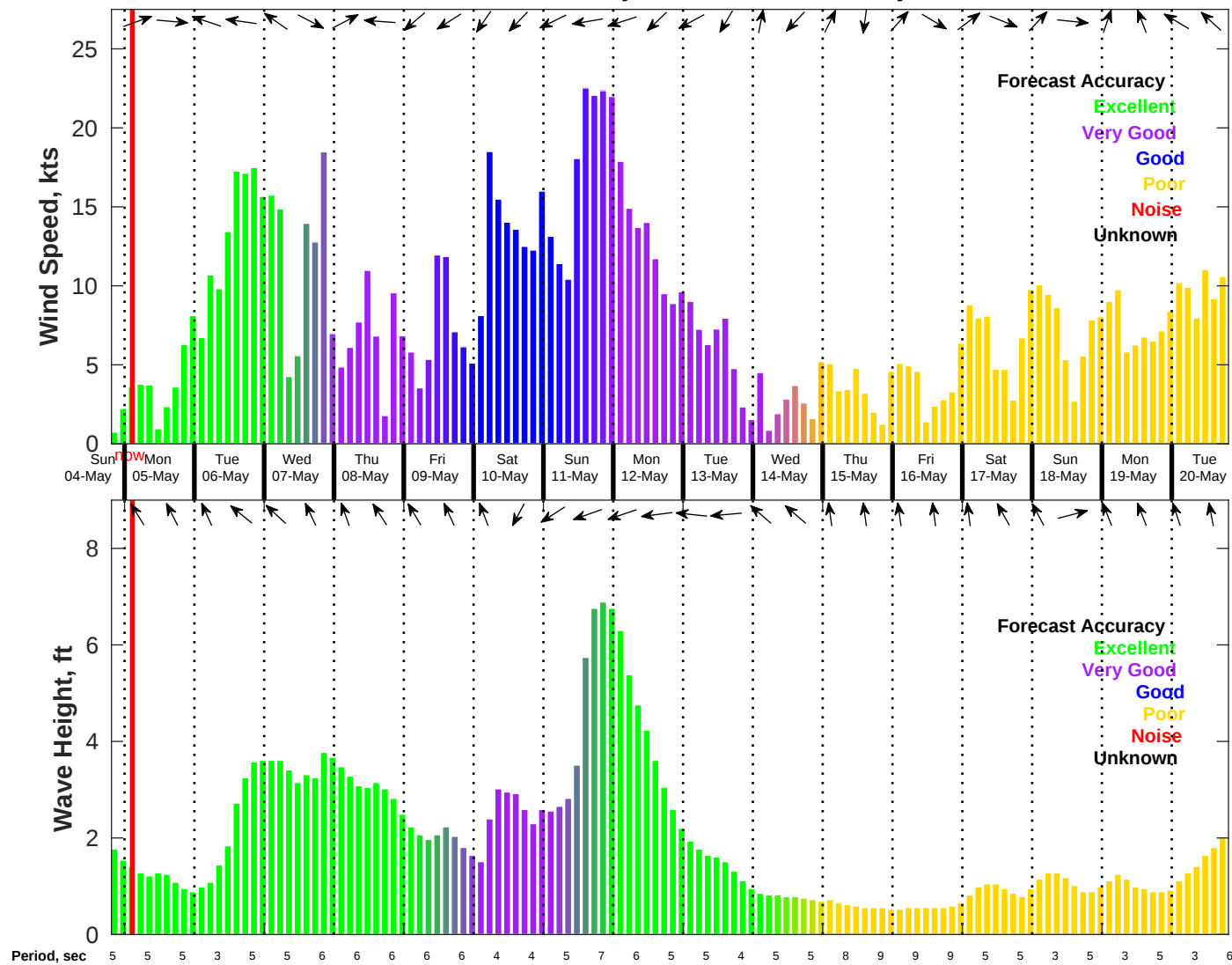
Wind & Wave Forecast for NDBC 42040 from 04-May-2025 19:00:00 to 20-May-2025 19:00:00
