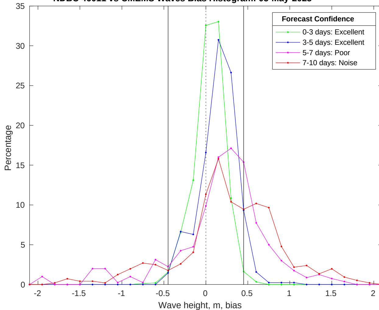
NDBC 46011 vs CMEMS Waves Bias Histogram: 05-May-2025
