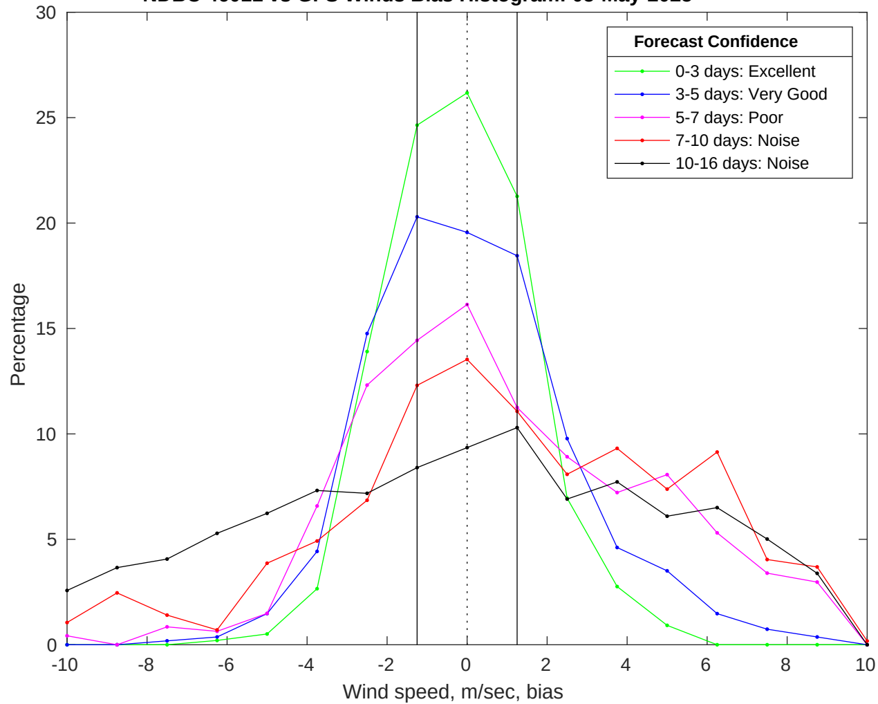
NDBC 46011 vs GFS Winds Bias Histogram: 05-May-2025
