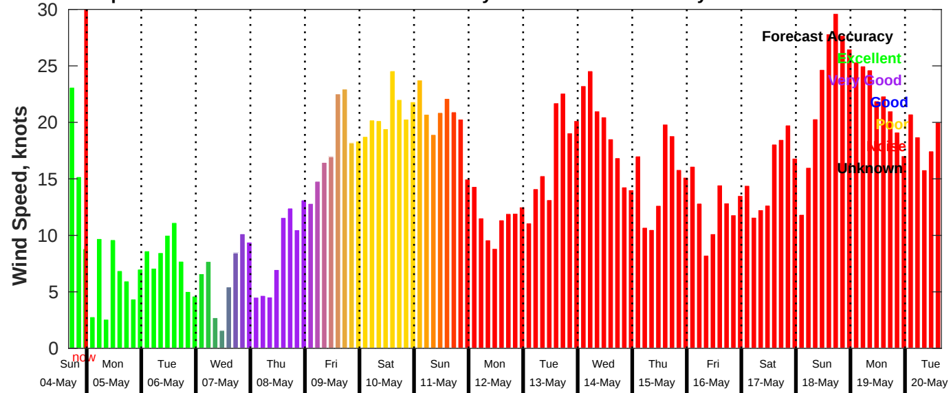
GFS Wind Speed Forecast for NDBC 46011 from 04-May-2025 16:00:00 to 20-May-2025 16:00:00
