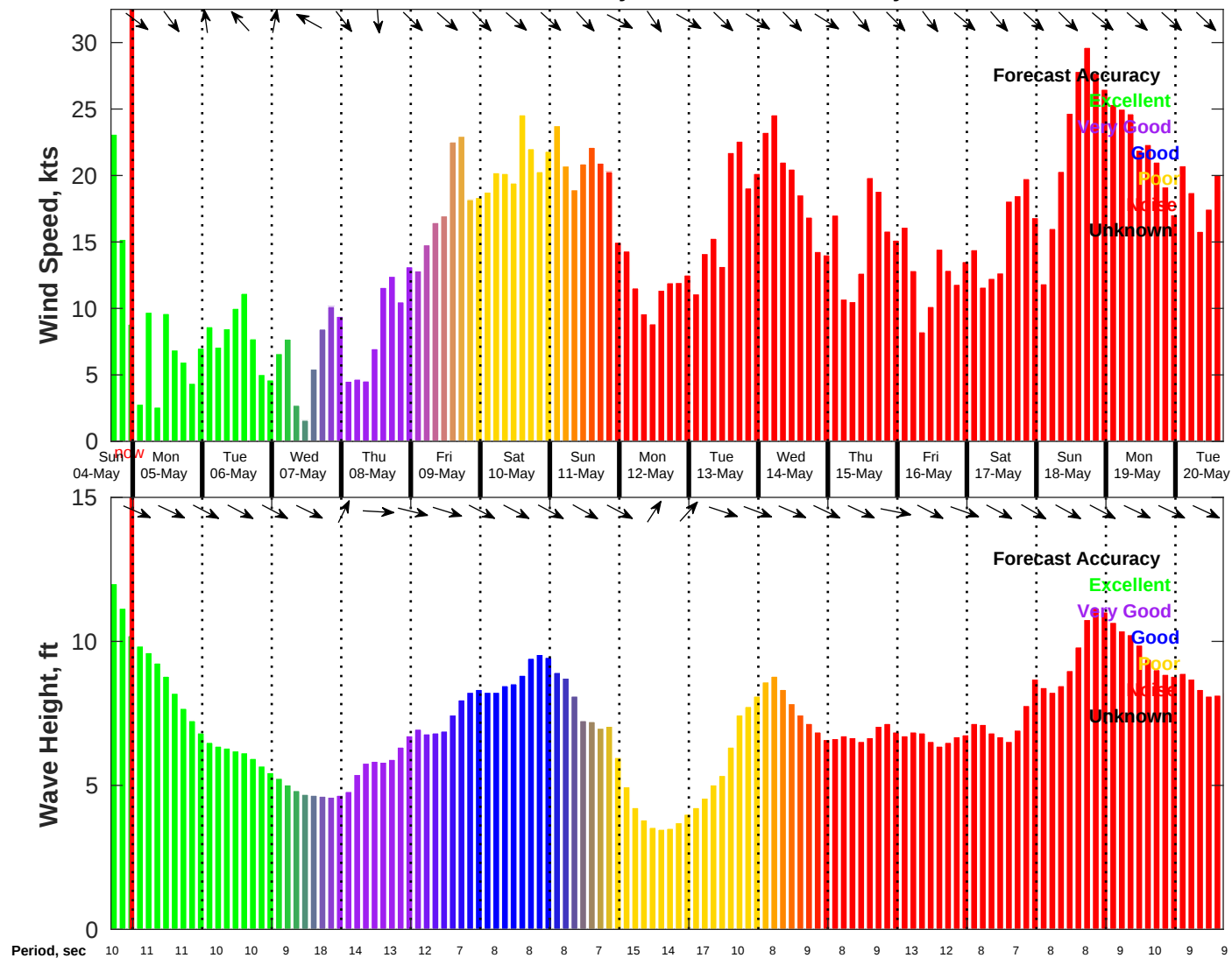
Wind & Wave Forecast for NDBC 46011 from 04-May-2025 16:00:00 to 20-May-2025 16:00:00
