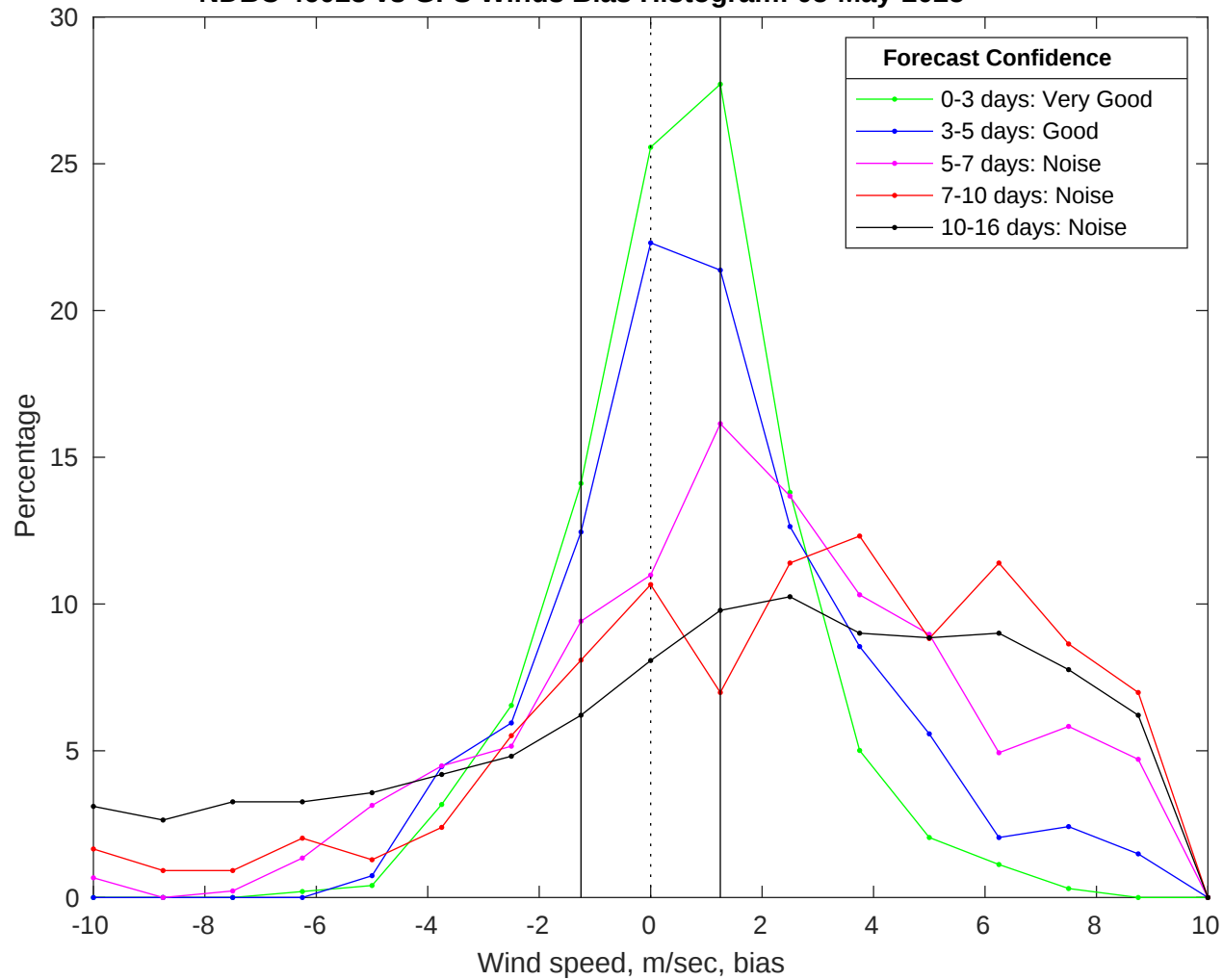
NDBC 46028 vs GFS Winds Bias Histogram: 05-May-2025
