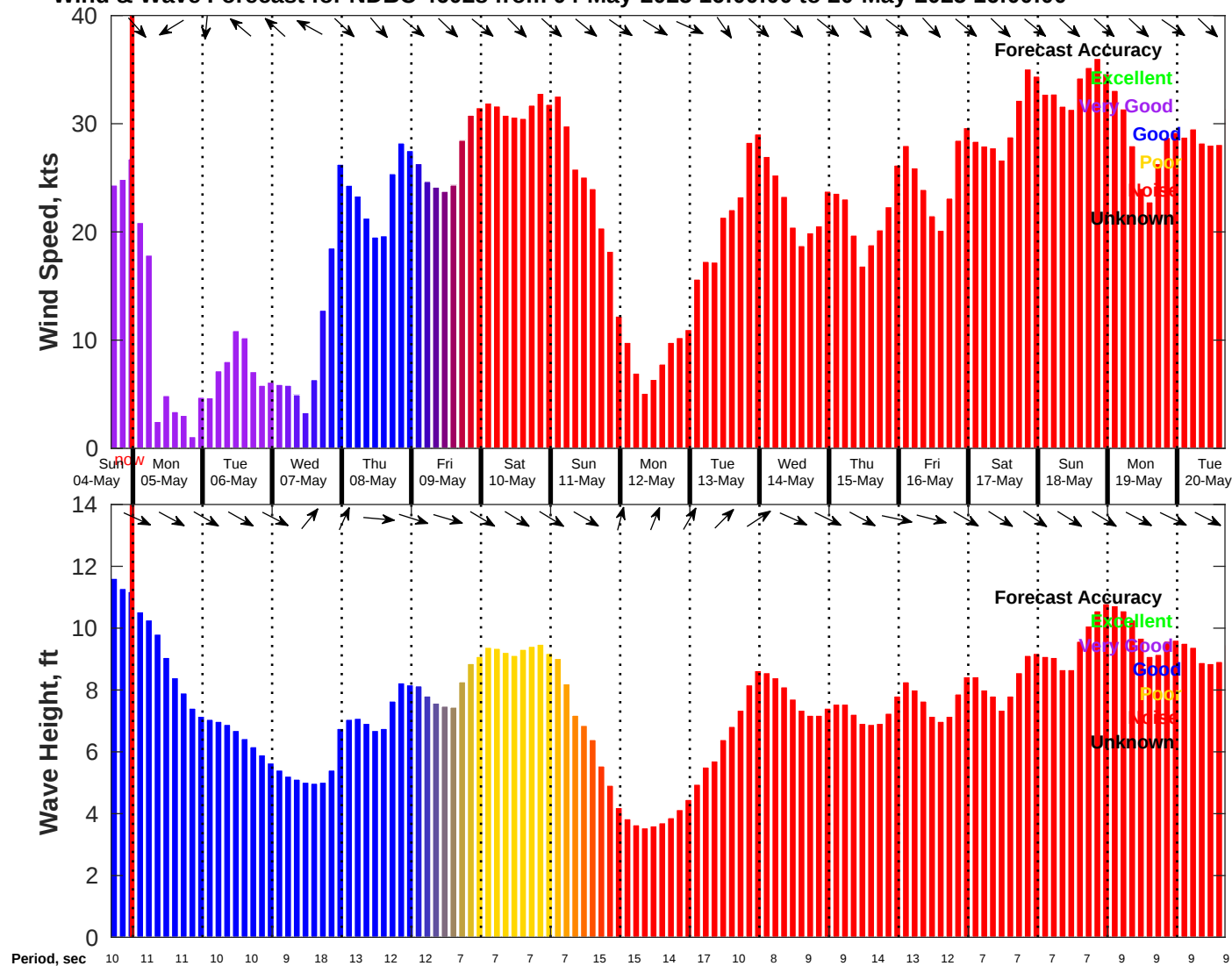
Wind & Wave Forecast for NDBC 46028 from 04-May-2025 16:00:00 to 20-May-2025 16:00:00
