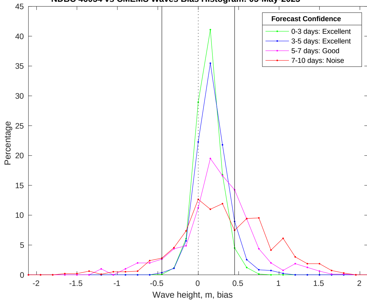
NDBC 46054 vs CMEMS Waves Bias Histogram: 05-May-2025
