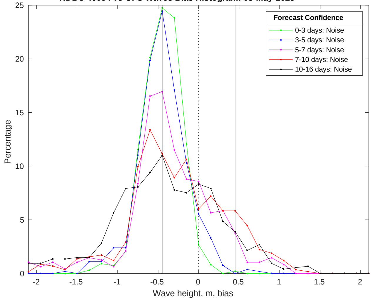
NDBC 46054 vs GFS Waves Bias Histogram: 05-May-2025
