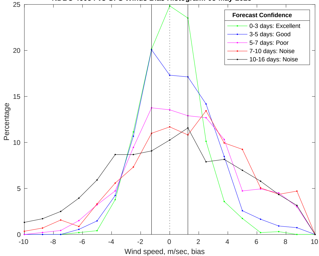
NDBC 46054 vs GFS Winds Bias Histogram: 05-May-2025
