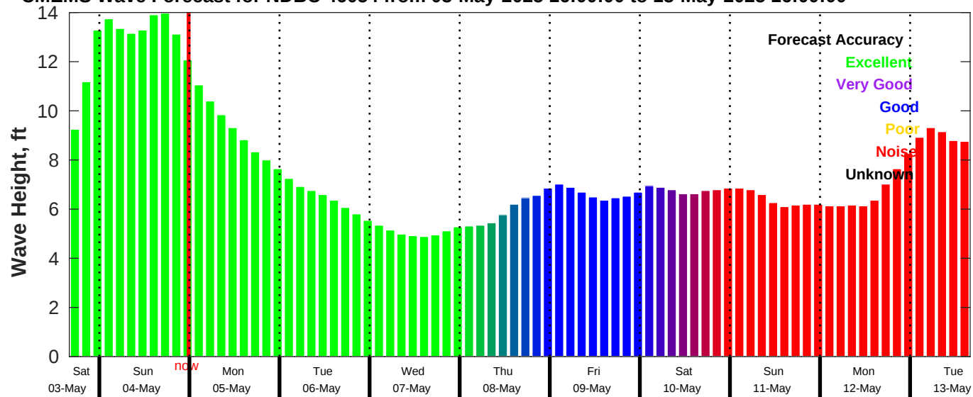
CMEMS Wave Forecast for NDBC 46054 from 03-May-2025 16:00:00 to 13-May-2025 16:00:00
