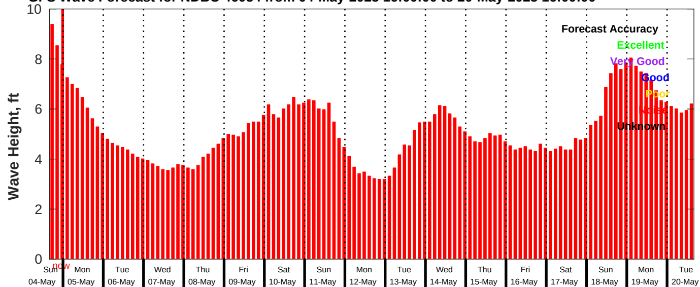
GFS Wave Forecast for NDBC 46054 from 04-May-2025 16:00:00 to 20-May-2025 16:00:00
