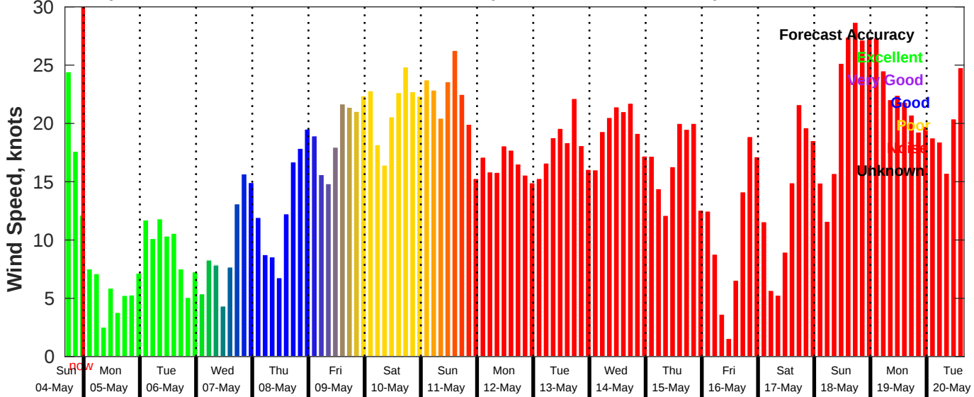
GFS Wind Speed Forecast for NDBC 46054 from 04-May-2025 16:00:00 to 20-May-2025 16:00:00
