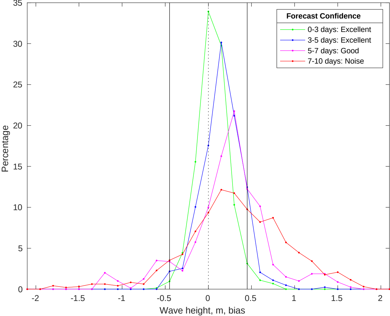
NDBC 46069 vs CMEMS Waves Bias Histogram: 05-May-2025
