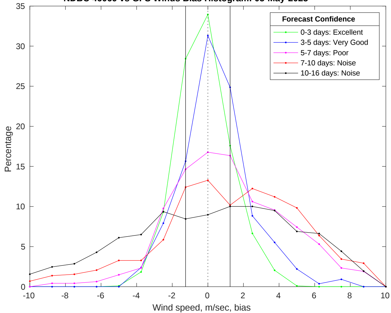
NDBC 46069 vs GFS Winds Bias Histogram: 05-May-2025
